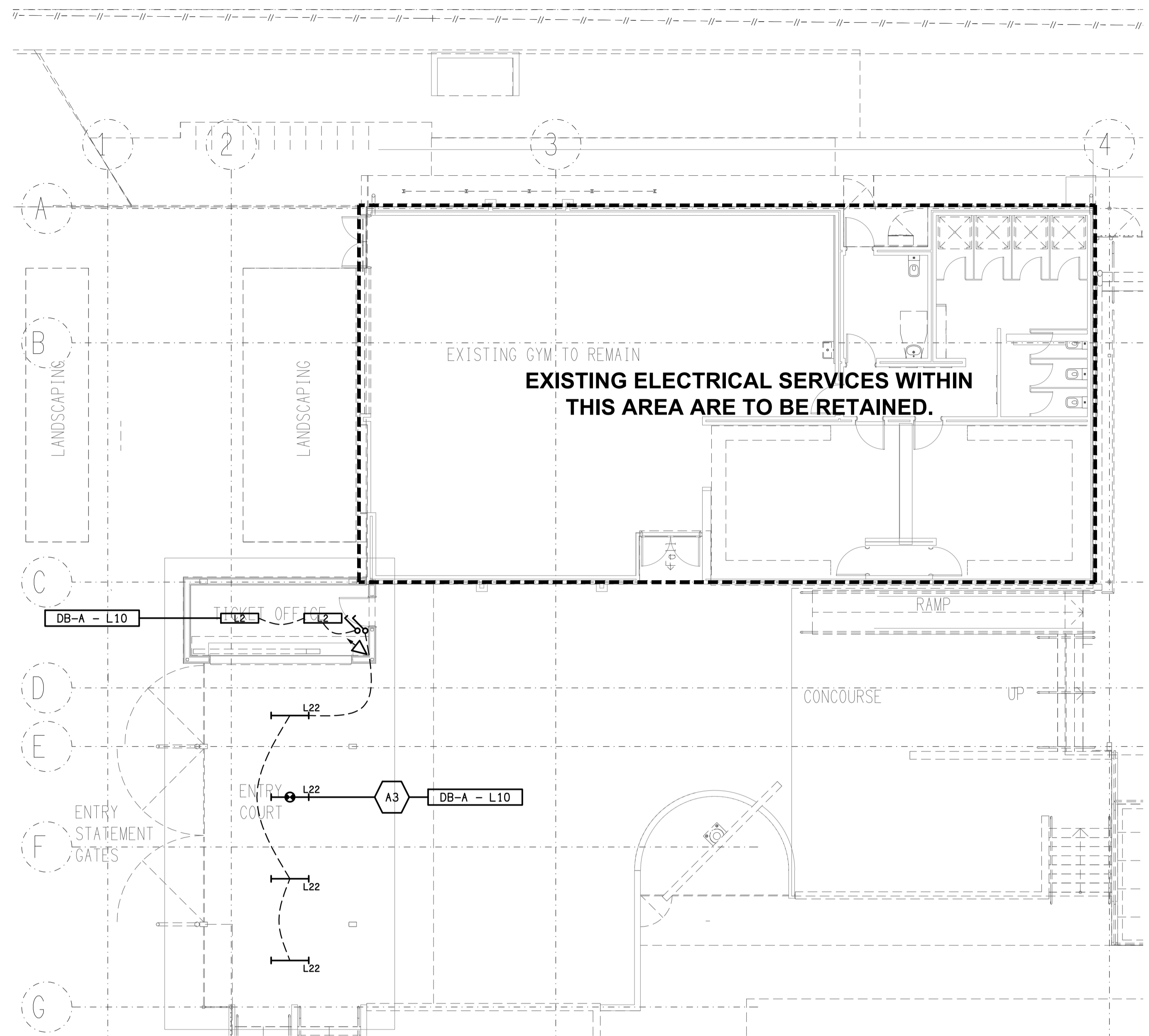
REFLECTED CEILING PLAN TICKET OFFICE SCALE 1:100
